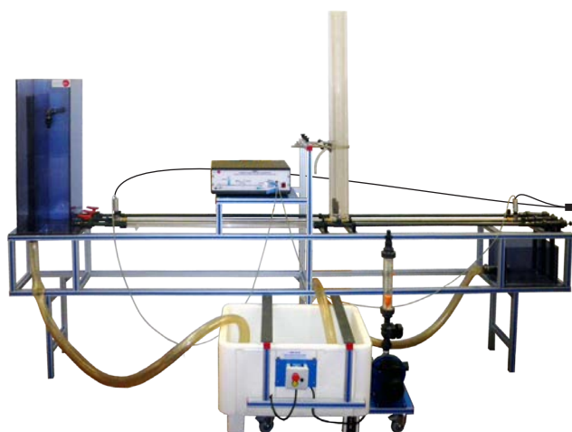
① Unit: EGAC. Computer Controlled Water Hammer Unit
