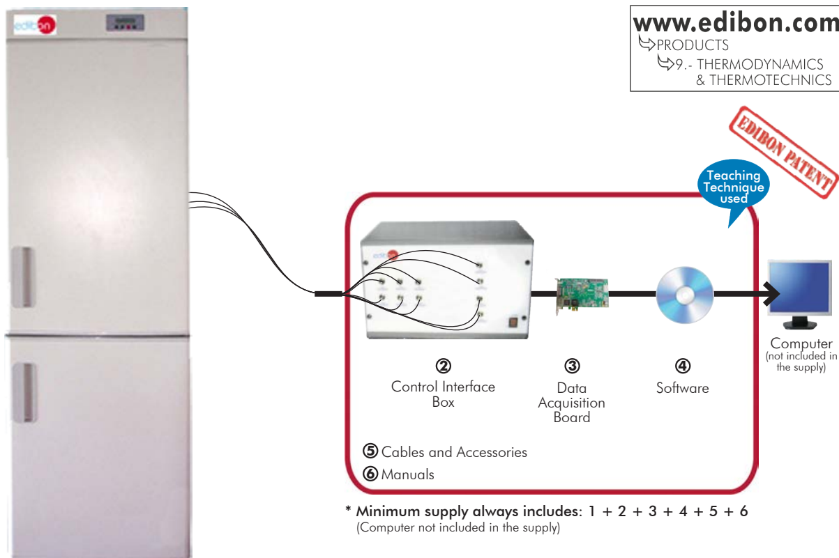
① Unit: TRD2PC. Two Doors Domestic Refrigeration System Trainer
