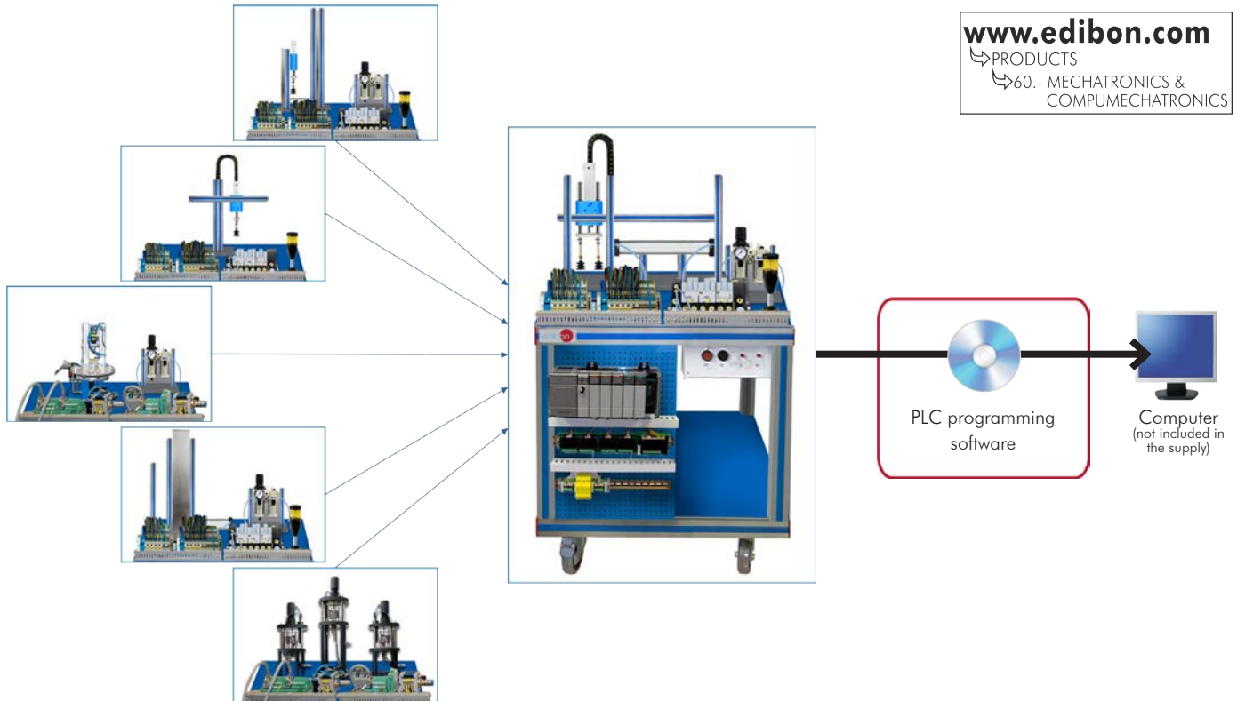
Unit: AE-PLC-MEMB. Bottling Workstation
