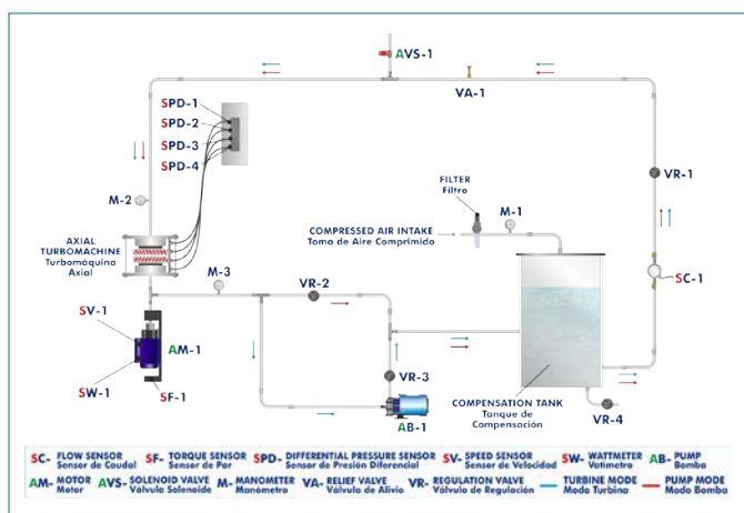
① Unit: HMFACT. Computer Controlled Axial Flow Turbomachines Unit
