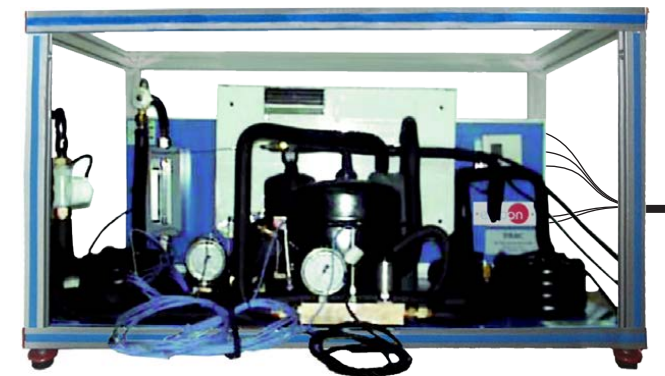
① Unit: THARL2C. Computer Controlled Refrigeration and Air Conditioning Unit (one condenser (water) and two evaporators (water and air))
