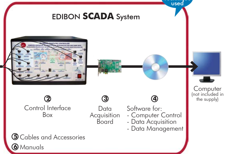
① Unit: THARL2C. Computer Controlled Refrigeration and Air Conditioning Unit (one condenser (water) and two evaporators (water and air))
