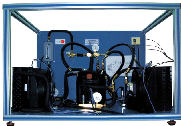
① Unit: THAAAC. Computer Controlled Air Conditioning Unit (one condenser (air) and one evaporator (air))
