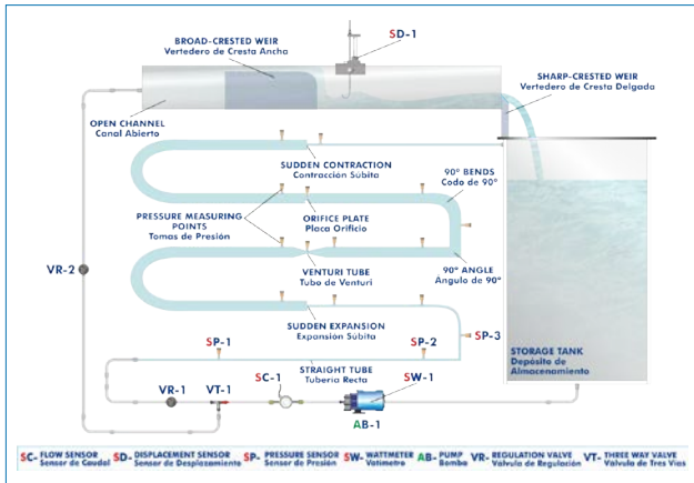
① Unit: WFPC. Computer Controlled Unit to Study Water Flow Principles
