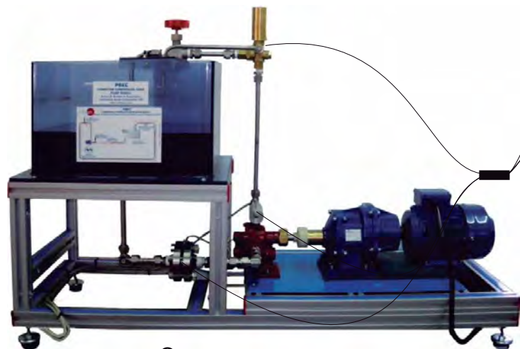
① Unit: PBECE. Gear Pump Bench
