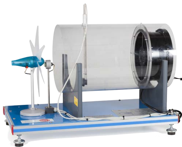
① Unit: MINI-EEEC. Computer Controlled Wind Energy Basic Unit
