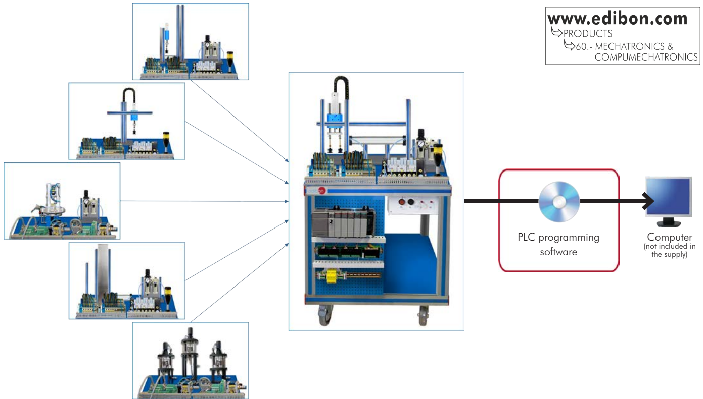
Unit: AE-PLC-MR4. Rotary Table Workstation 4
