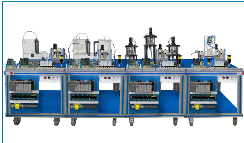
① Unit: AE-PLC-FMS4. Flexible Manufacturing System 4
