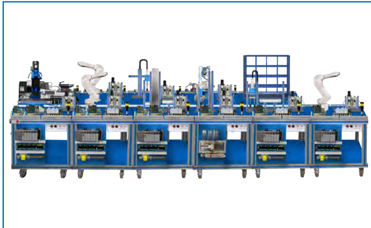
① Unit: AE-PLC-FMS12. Flexible Manufacturing System 12
