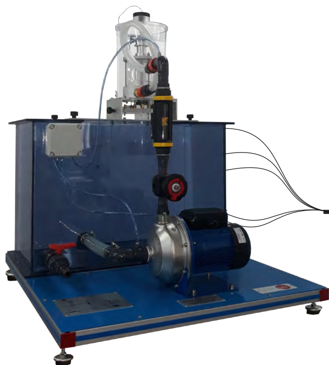
① Unit: TKC. Computer Controlled Kaplan Turbine
