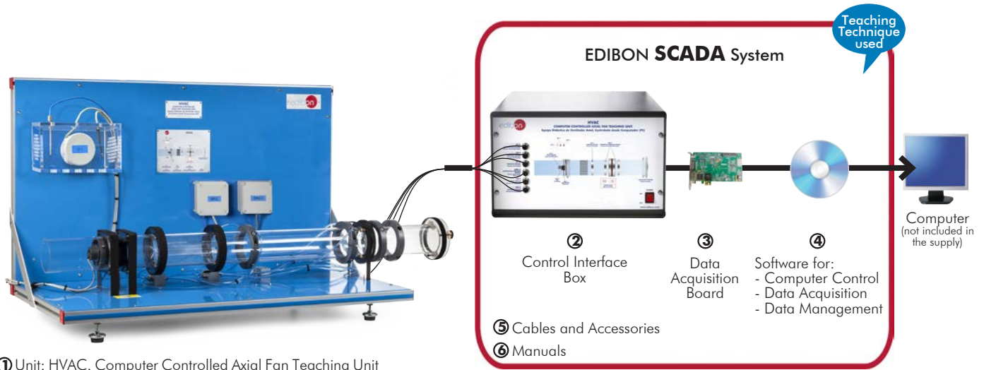
① Unit: HVAC. Computer Controlled Axial Fan Teaching Unit
