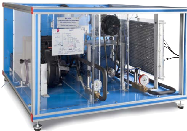
① Unit: TAAUC. Computer Controlled Automobile Air Conditioning Unit
