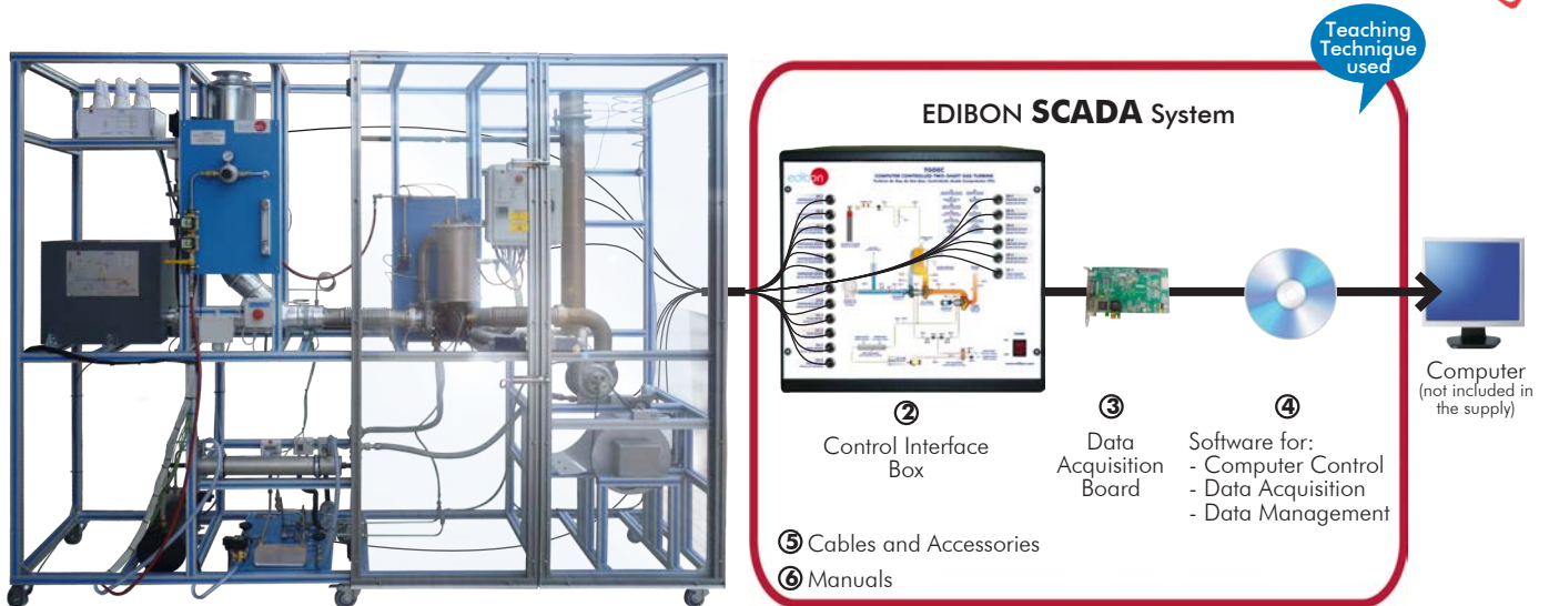
① Unit: TGDEC. Computer Controlled Two -Shaft Gas Turbine
